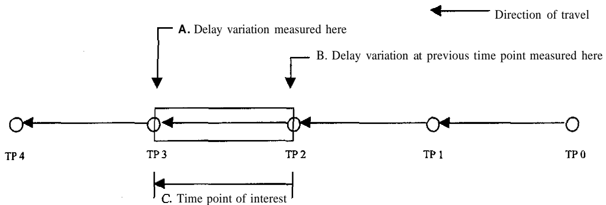
Figure 5.3: Model Structure
