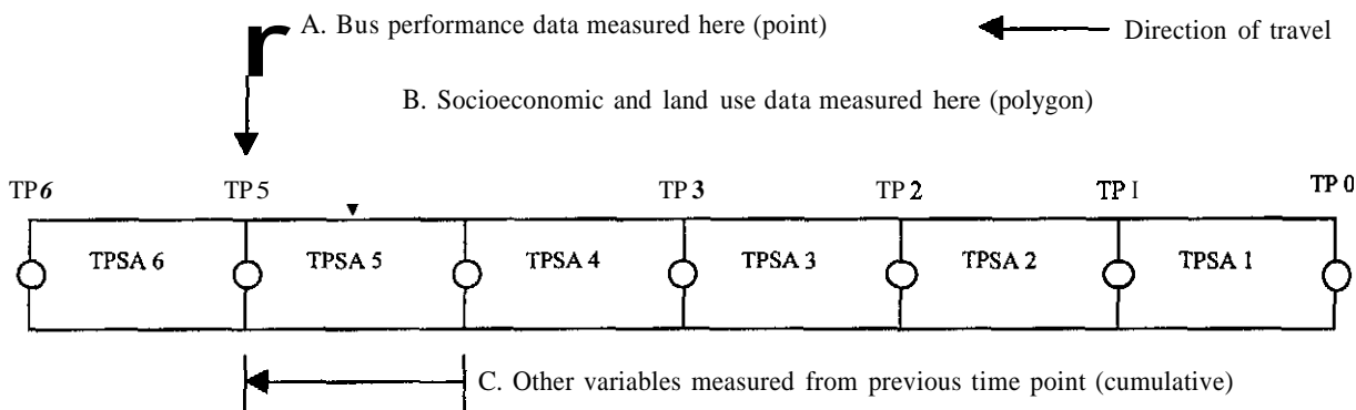
Figure 5.2: Data Consistency
