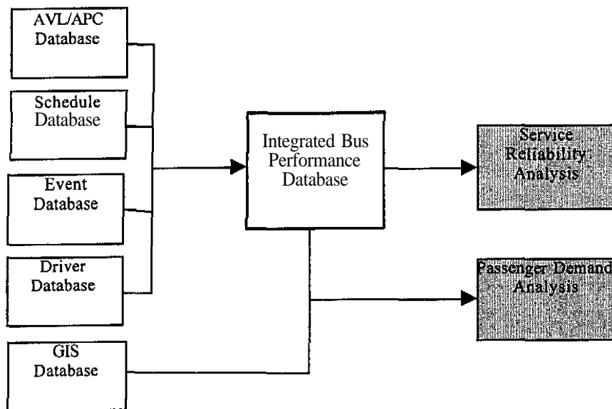
Figure 5.1: Database Integration
