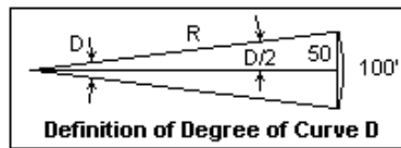
Figure 3-3 Definition of degree of curvature (Source: Calvert, 2004)
