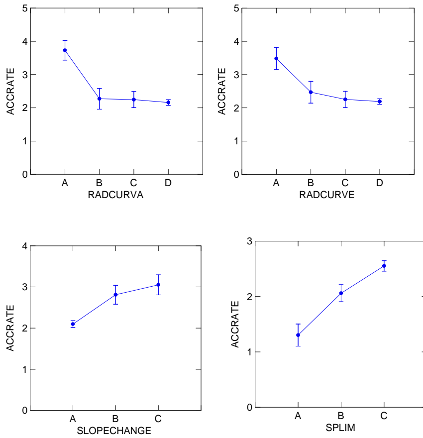
Figure 4-34 Impact of each variable on accident rate in F-test
