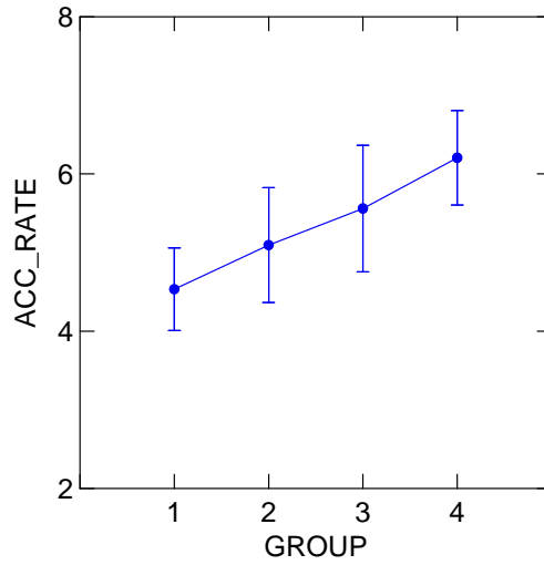
Figure 4-33 ANOVA test result for effect of gradation on accident rate
