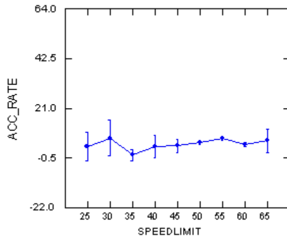
Figure 4-29 Accident rates on curvy segments with different speed limits
