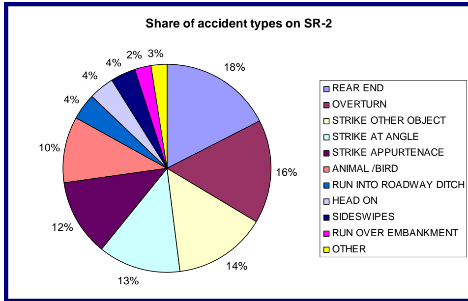
Figure 4-2 Shares of accident types on SR-2
