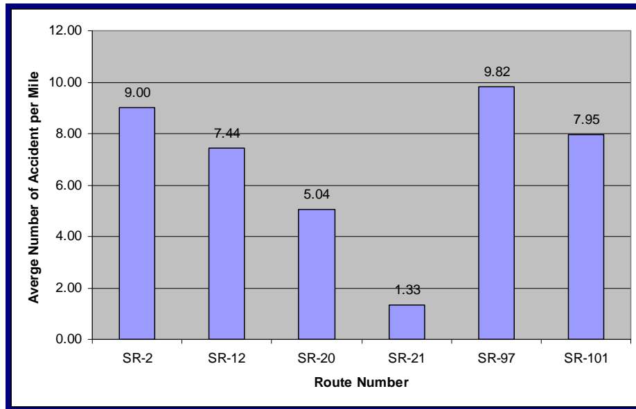
Figure 4-8 Average numbers of accidents per mile by route
