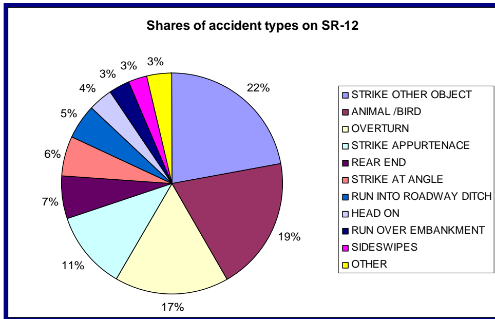
Figure 4-3 Shares of accident types on SR-12
