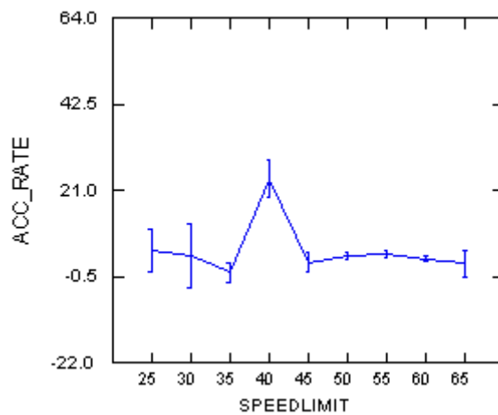
Figure 4-31 Accident rates on straight segments with different speed limits
