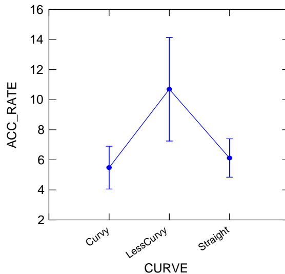
Figure 4-28 Accident rate on segments with different curvy levels
