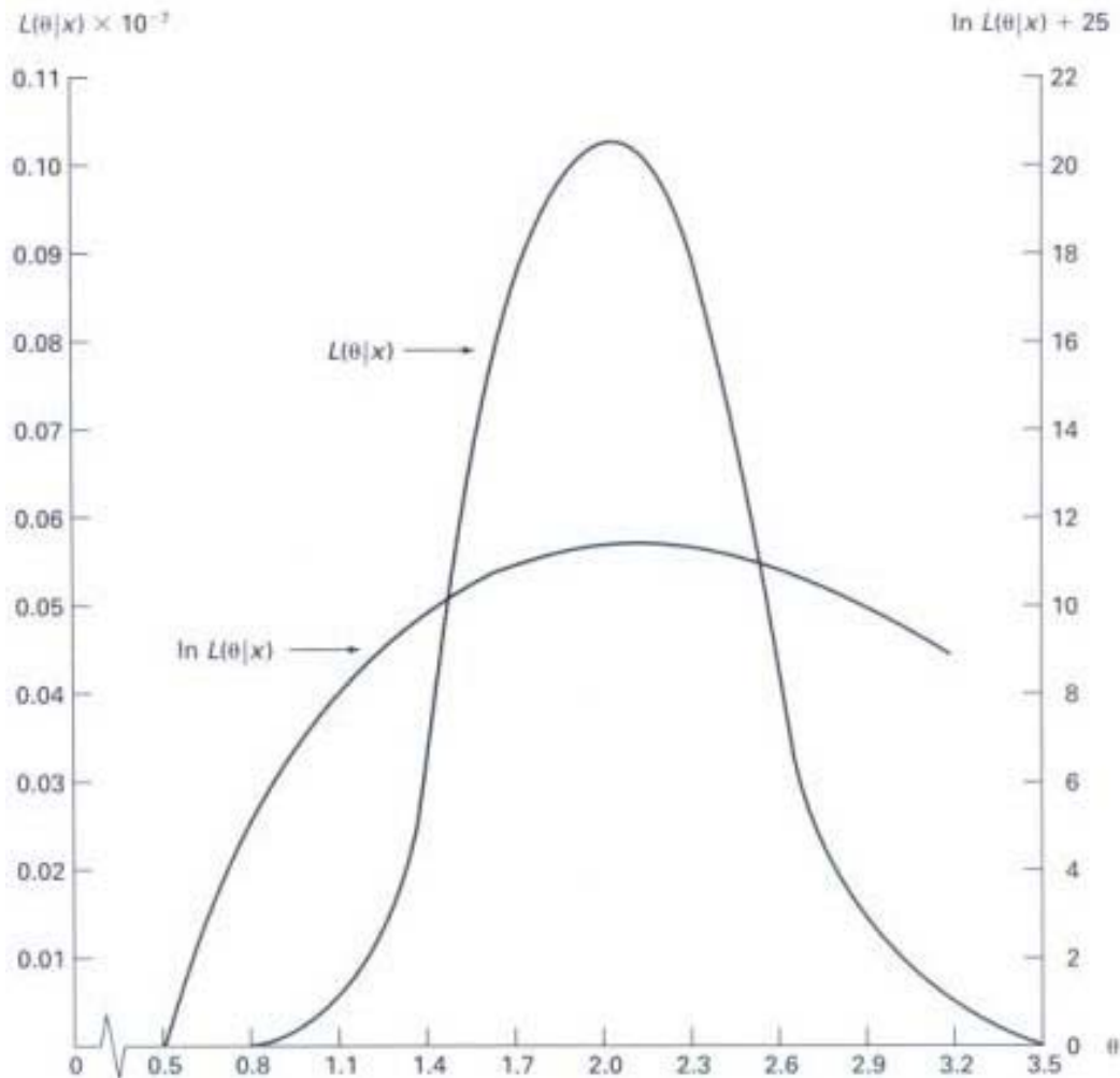
Figure 3-6 Likelihood and log likelihood functions for the Poisson distribution. [Source: Greene (2000)]
